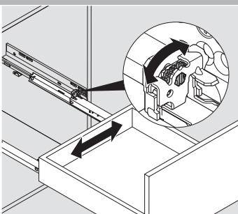
Balance side adjustment via the right, back runner
