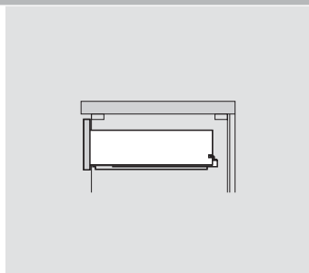
Depth adjustment \pm 2 mm MOVENTO with TIP-ON
