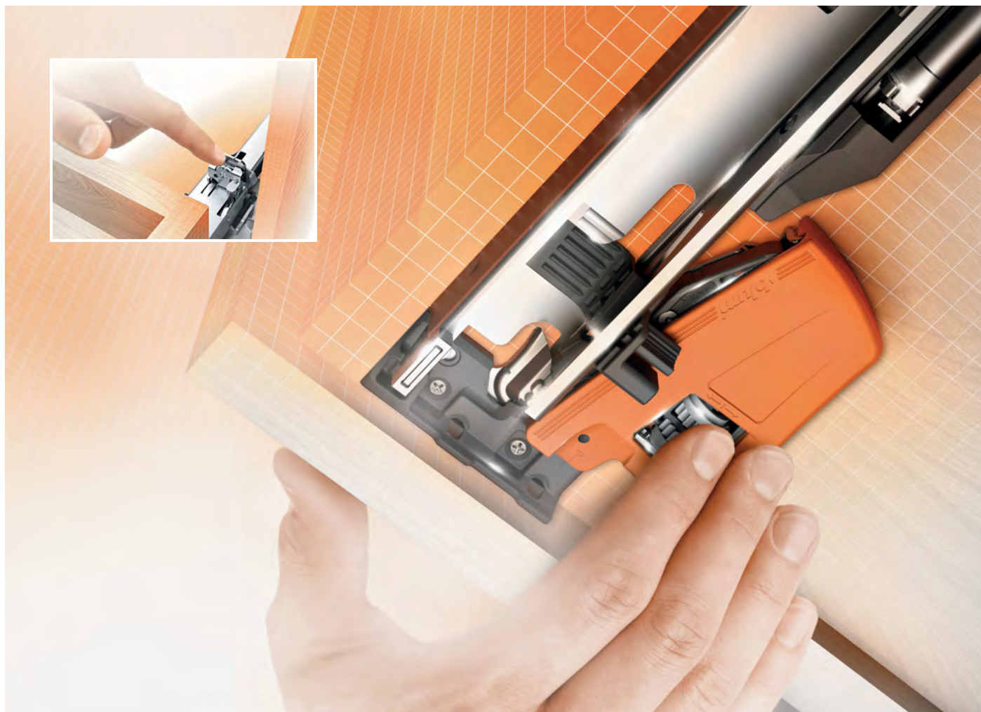
1 Side adjustment – carried out via the locking device, a correction to the side adjustment is carried out, if required, behind the runner.
