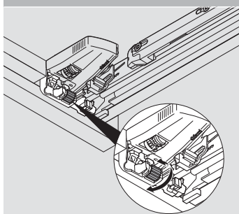
Depth adjustment \pm 2 mm MOVENTO with BLUMOTION
