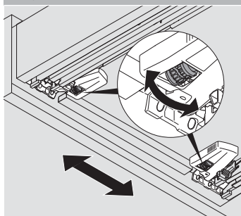
Side adjustment on both sides via the locking device \pm 1.5 mm*
